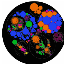
Pebbles Treemap
